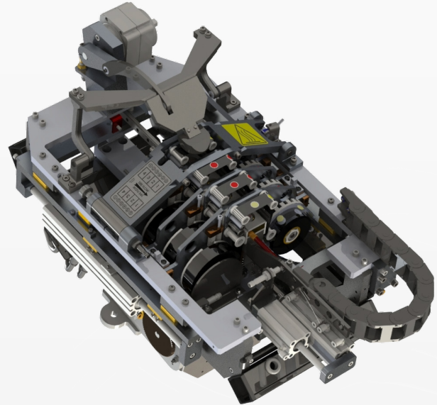
AkroMARK™ DUO Bottom View
