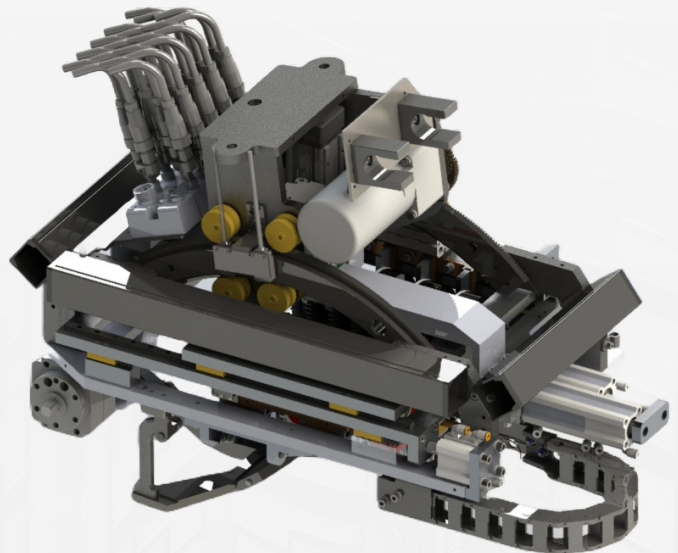
AkroMARK™ DUO Top View
